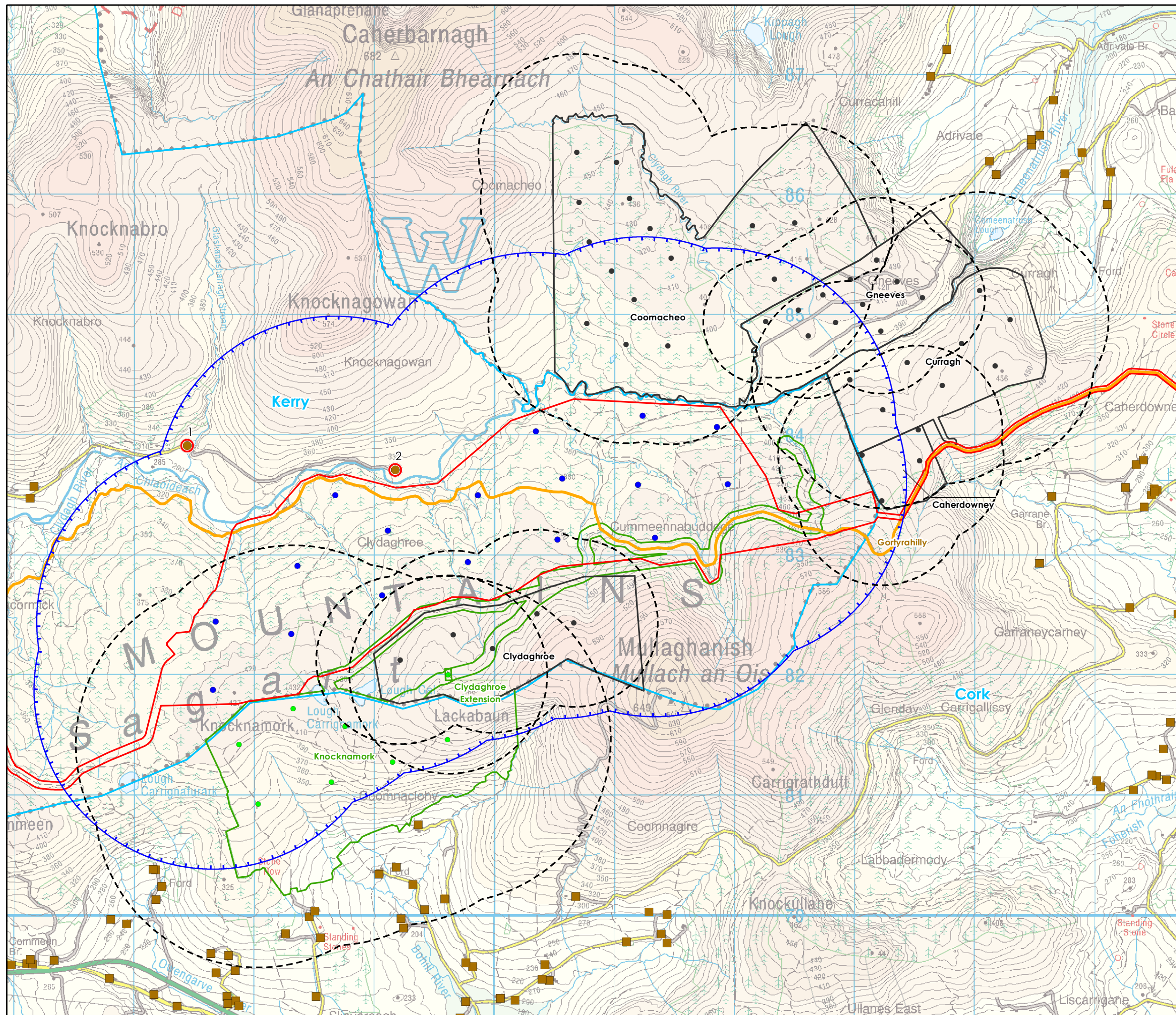
Figure 15-2b Cumulative shadow flicker extents and Minimum Rotor Diameter
